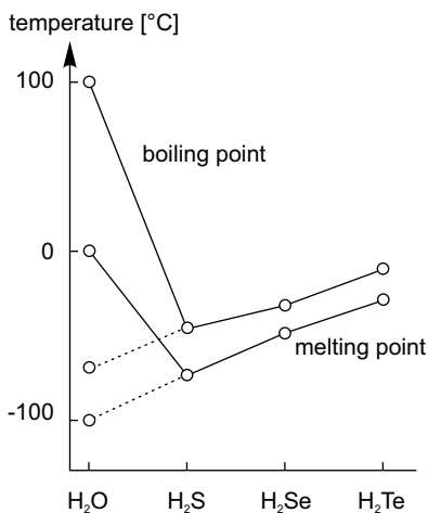
Figure 1.5 Melting and boiling temperatures of hydrogen compounds in the oxygen group of the periodic table and the expected values for H 2 O.
