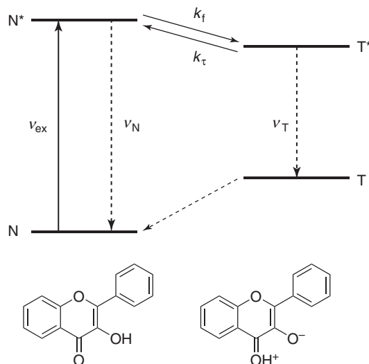
Figure 1.12 3-Hydroxyflavone (flavonol) exhibits ESIPT as a result of motion of the OH proton to the nearby oxygen in the excited state. (a) The generic level scheme used to describe this type of reaction. In the flavones, often both compounds are present in the excited state, and dual emission can occur, leading to the possibility of using the color change as indicator. The forward and reverse rates ( k_f and k_r ) in the excited state are usually much faster than
