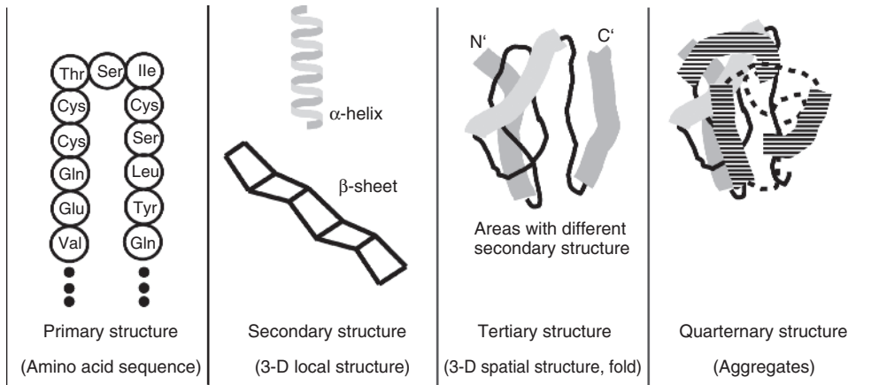
Figure 1.13 Protein structures.
