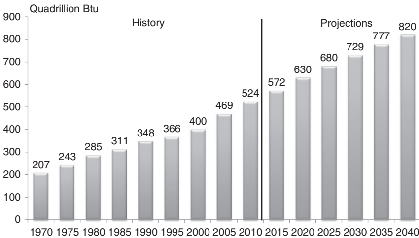
Figure 1.2 World primary energy consumption, 1970–2040 in units of (a) petawatt-hours; (b) Btu (British thermal units). Source: Based on data from: Energy Information Administration (EIA), International Energy Outlook 2013.
