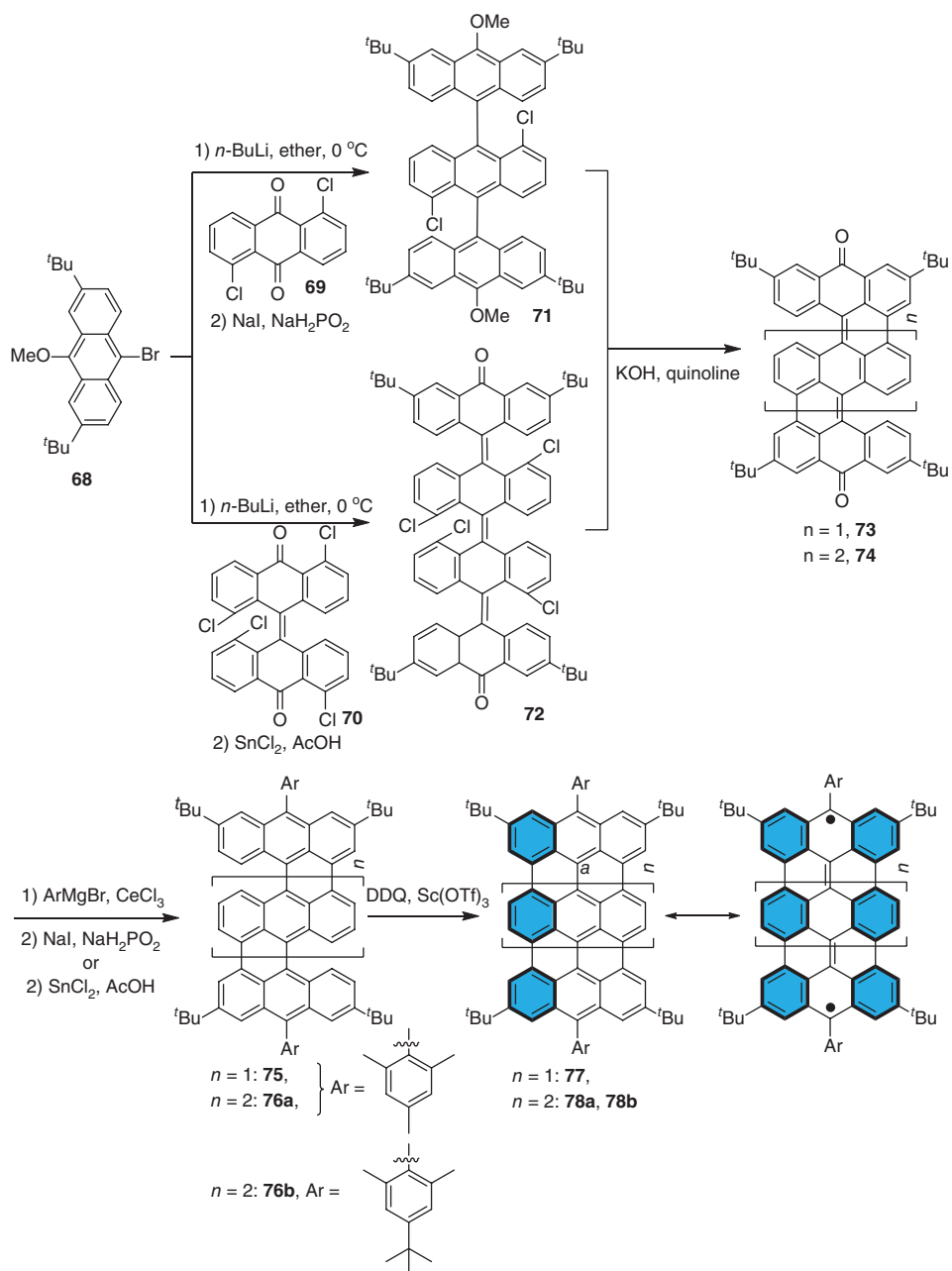
Figure 1.13 Syntheses of teranthene and quarteranthene derivatives.
