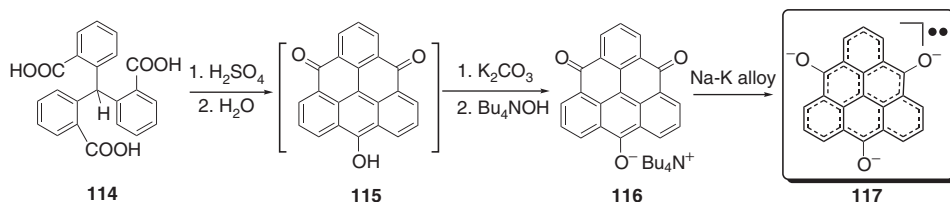
Figure 1.22 Synthesis of the biradical trianion 117 .
