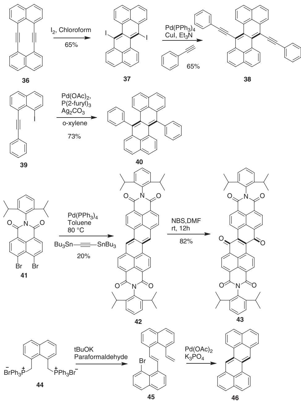
Figure 1.7 Synthesis of zethrene derivatives.
