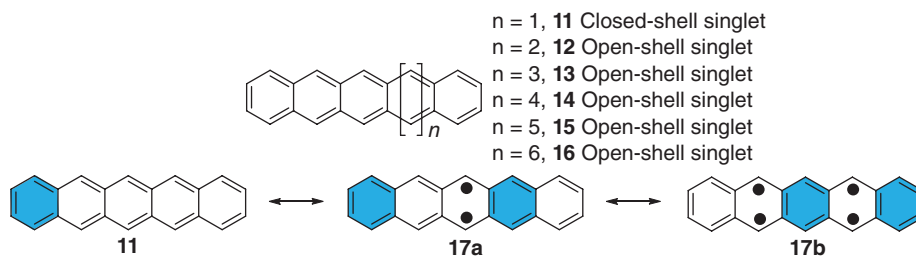
Figure 1.2 Resonance forms of pentacene 11 .
