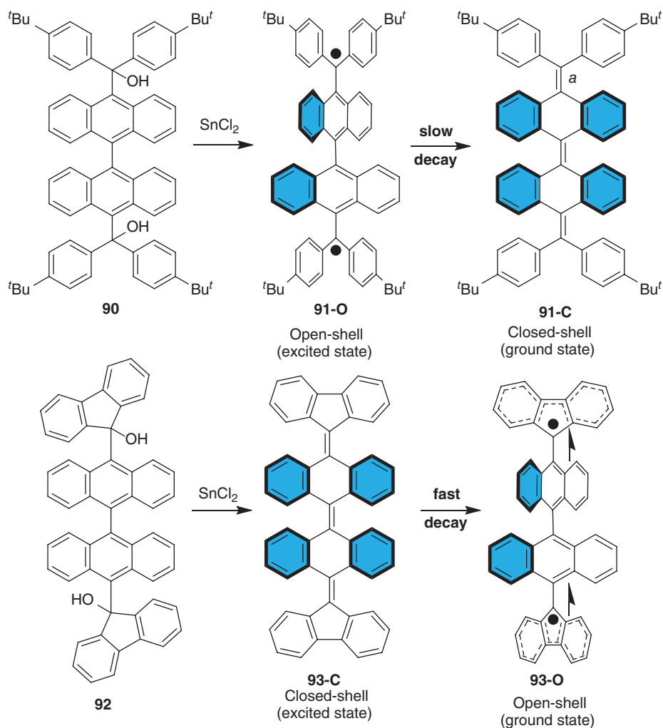
Figure 1.17 Tetrabenzo-Tschitschibabin's hydrocarbons.
