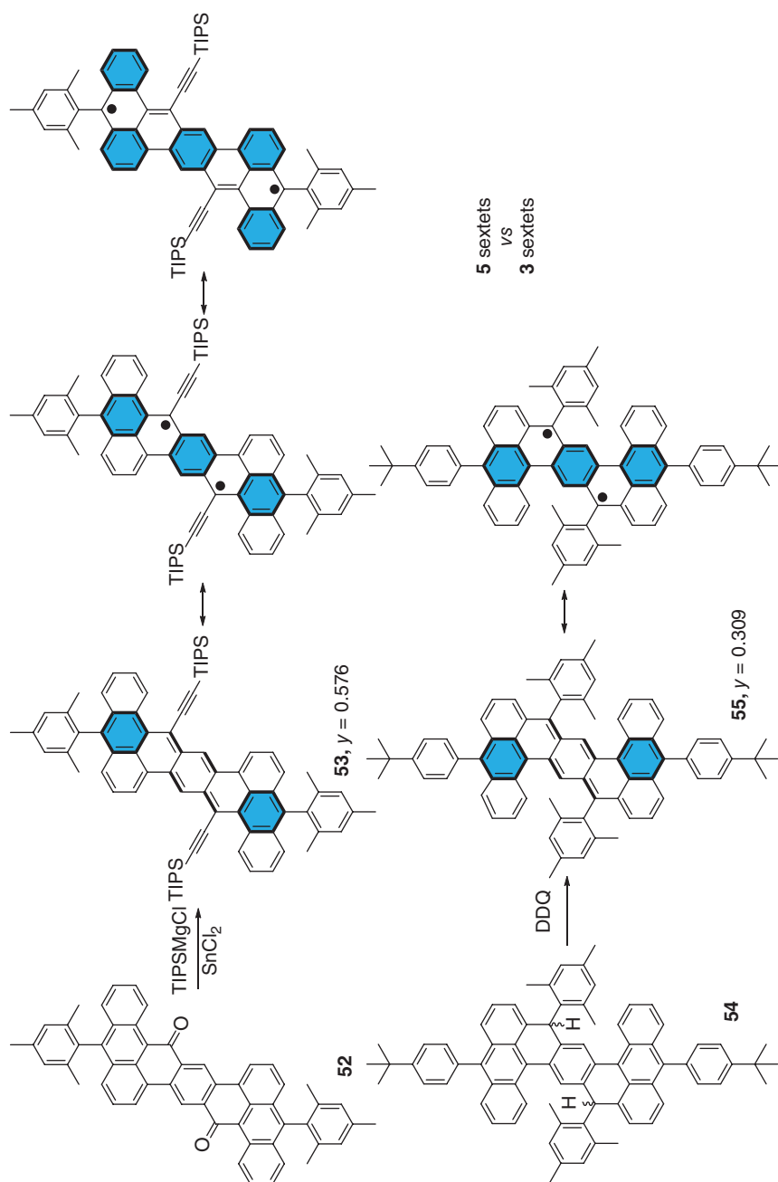
Figure 1.9 Exercise of Clar's sextet rule in isomeric dibenzoheptazethrene systems.
