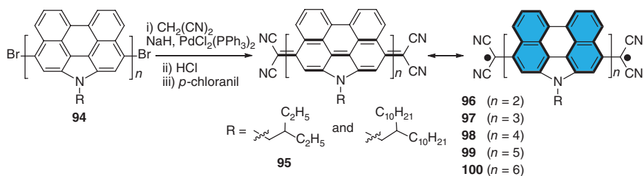
Figure 1.18 Tetracyano-N-annulated perylene quinodimethanes.
