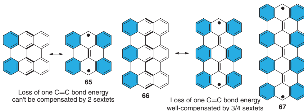
Figure 1.12 Structures of anthenes.
