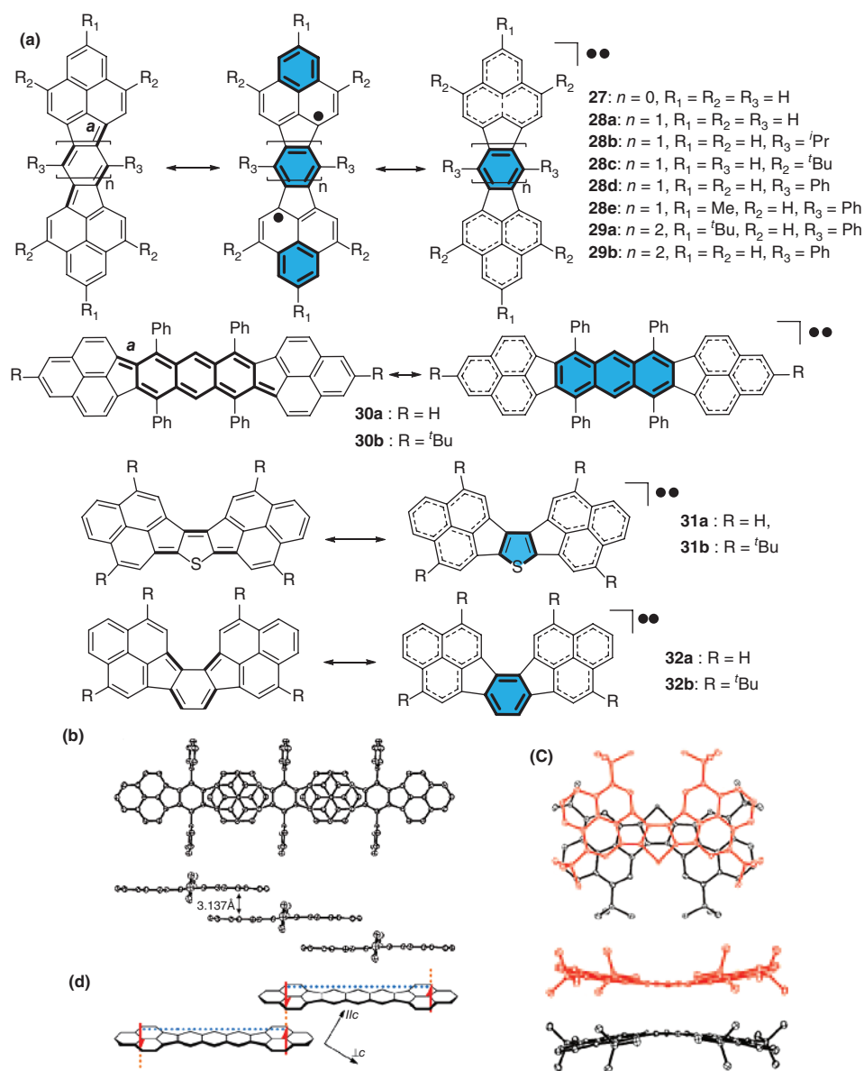
Figure 1.4 (a) Resonance forms of bis(phenalenyl)s with different aromatic linkers. (b) Crystal structure of 28d . (Adapted with permission from Ref. [33]. Copyright 2005, John Wiley and Sons.) (c) Crystal structure of 31b . (Adapted with permission from
