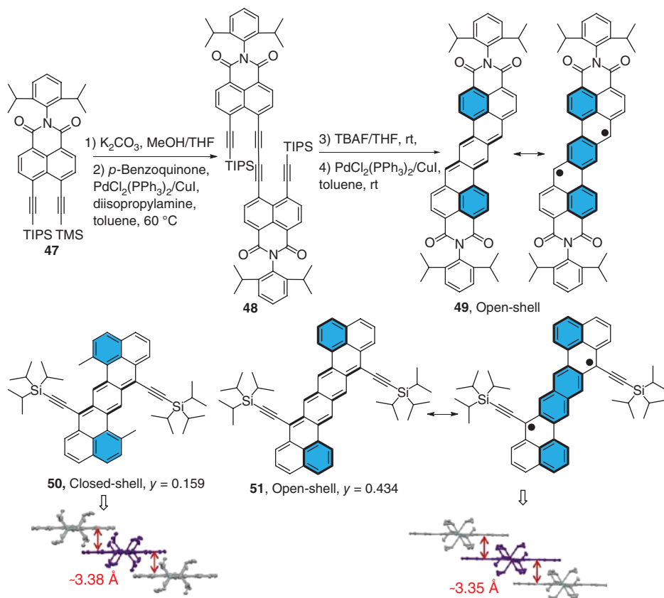
Figure 1.8 Heptazethrene and octazethrene derivatives. (Crystal figures are adapted with permission from Ref. [49]. Copyright 2012, American Chemical Society.)
