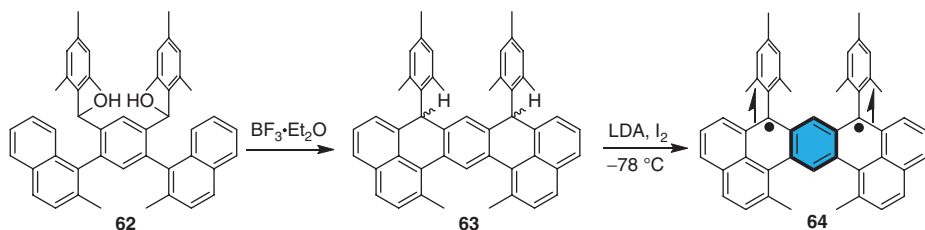
Figure 1.11 A persistent triplet biradical based on isomeric heptazethrene.
