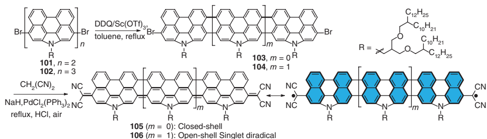
Figure 1.19 Fused tetracyano-N-annulated rylene quinodimethanes.
