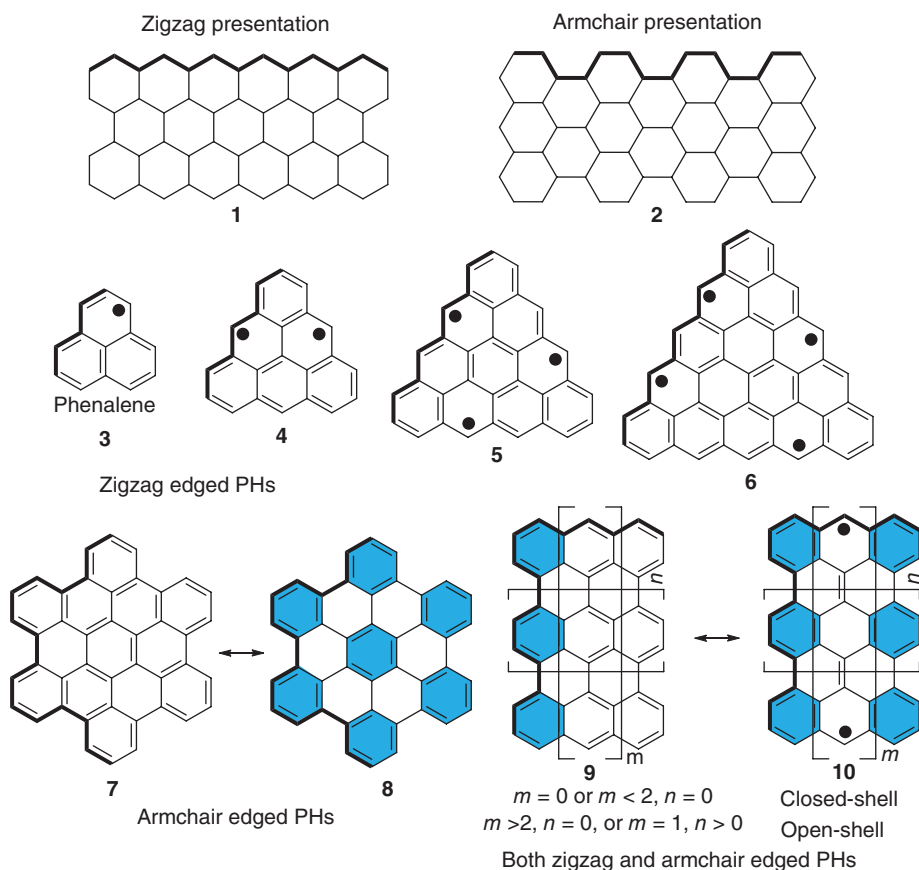
Figure 1.1 Molecular graphenes by fusion of benzene rings in different modes.
