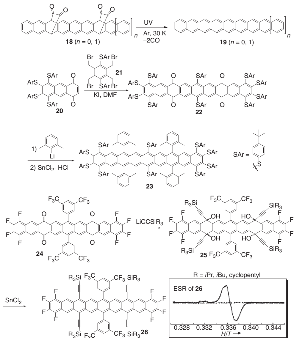
Figure 1.3 Nonacene derivatives. (ESR spectra of 26 is adapted with permission from Ref. [27]. Copyright 2011, John Wiley and Sons.)
