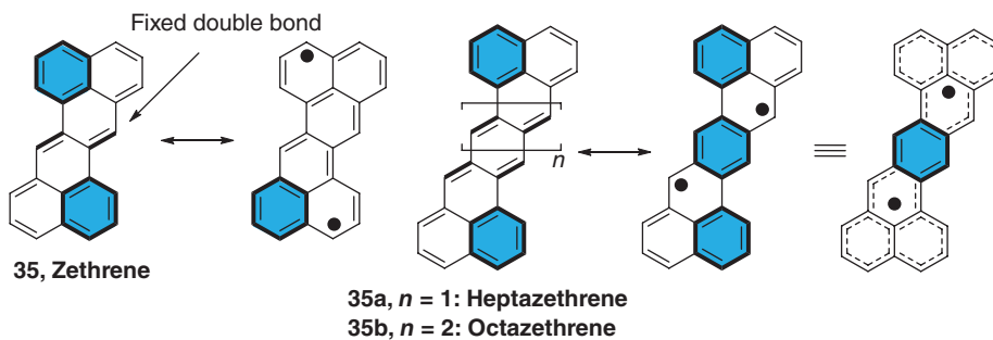
Figure 1.6 Resonance structures of zethrene and higher order zethrenes.
