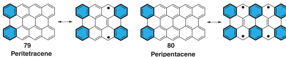
Figure 1.14 Structures of periacenes.
