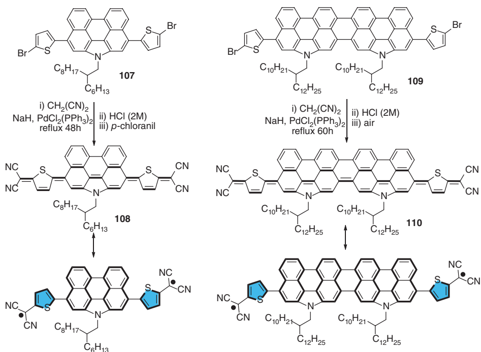
Figure 1.20 Tetracyanothiophene-capped N-annulated perylene quinodimethanes.
