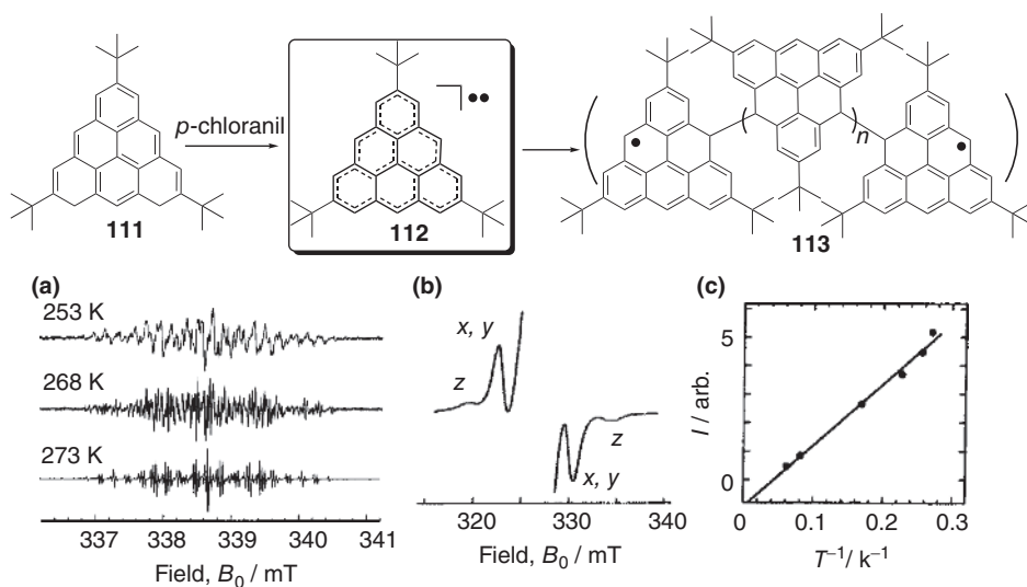
Figure 1.21 Synthetic route to tri- tert -butyl triangulene biradical 113 and its characterization by variable-temperature ESR spectroscopy. (Adapted with permission from Ref. [71]. Copyright 2001, American Chemical Society.)
