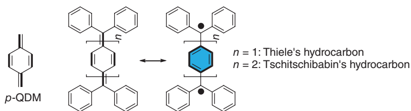
Figure 1.16 Parent p -QDM and its derivative.
