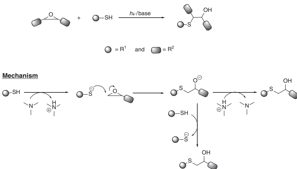
Scheme 1.13 Base catalyzed thiol–epoxy ring-opening click reaction.
