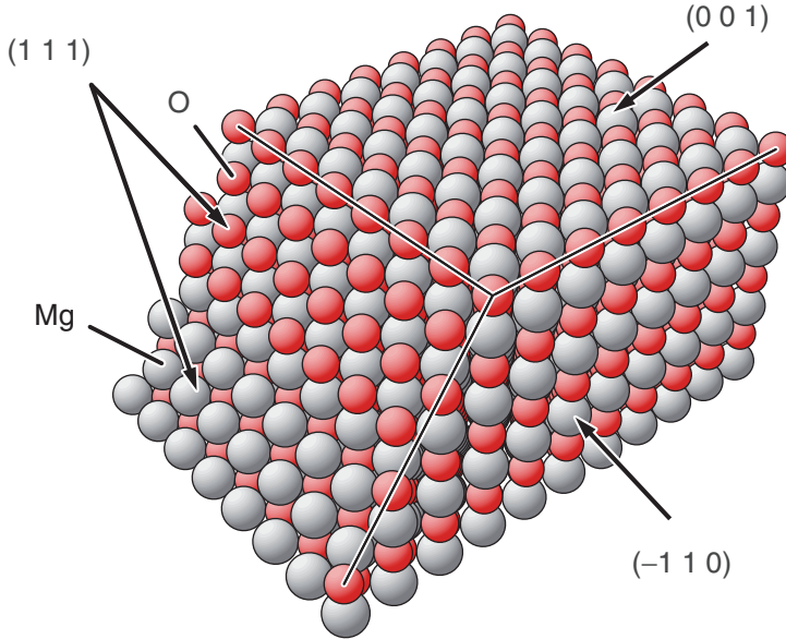
Figure 1.1 Section of an MgO crystal (NaCl lattice). The atoms are shown as shaded balls of different color and labeled accordingly. The section is enclosed by nonpolar (0\ 0\ 1) , (-1\ 1\ 0) , and by polar (1\ 1\ 1) oriented surfaces.
