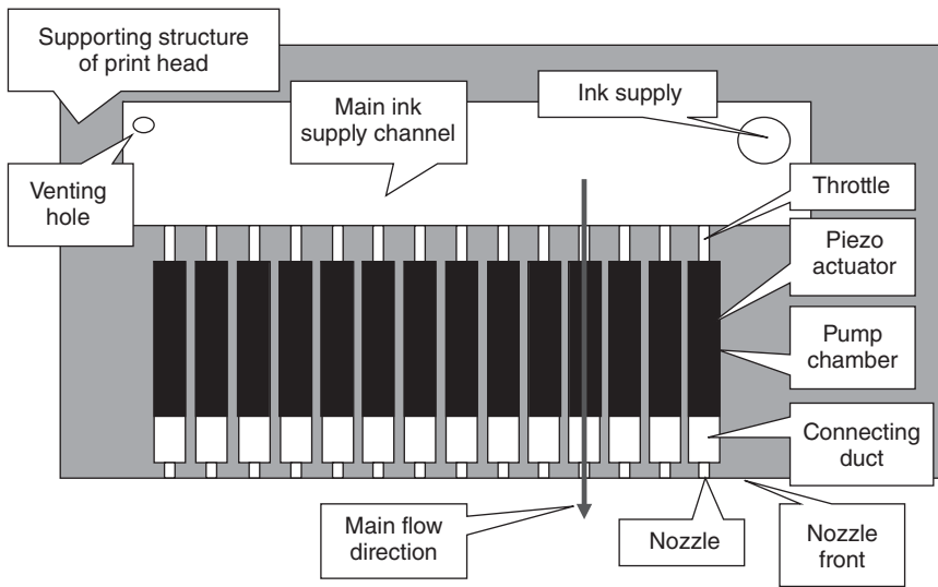
Figure 1.1 Schematic of piezo-driven print head of the Helmholtz type.
