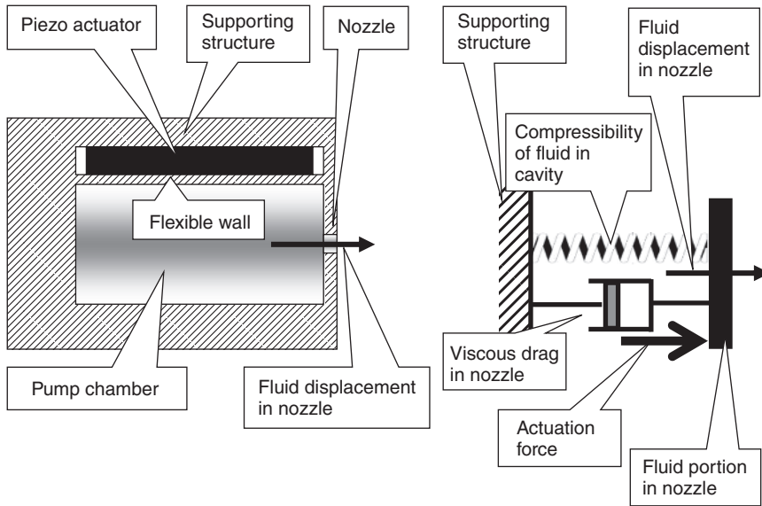
Figure 1.5 Single degree of freedom Helmholtz resonator modelled as a single mass–spring–damper oscillator. The spring models the compressibility of the fluid contained in the pump chamber, the damper is the viscous drag of the ink moving through the nozzle, and the mass is the fluid in the nozzle. By actuation a pressure is built up loading the mass in the nozzle by a force (pressure times surface area nozzle).
