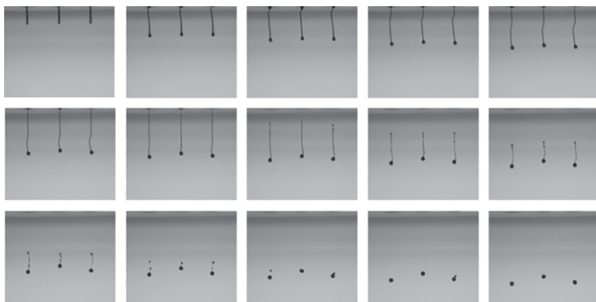
Figure 1.4 Jetting of a viscoelastic ink. Series of photographs showing the evolution of the droplet formation of a viscoelastic ink from a Dimatix Galaxy 256 nozzle print head with 30\text{ }\mu\text{m} diameter nozzles [7]. The pitch between nozzles is 254\text{ }\mu\text{m} ; the timing starts at 10\text{ }\mu\text{s} after the leading edge of the pulse, followed by images 10\text{ }\mu\text{s} apart in time. The shear viscosity of the ink has been tuned to 10\text{ mPa s} . The surface tension measures 30\text{ mN m}^{-1} . The final droplet volume equals 15\text{ pl} , its speed 2\text{ m s}^{-1} .
