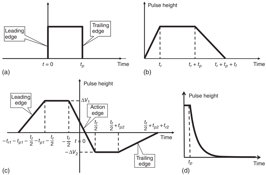
Figure 1.6 Different pulse shapes. (a) square pulse. (b) asymmetric trapezoidal pulse with different rise and fall times. (c) asymmetric double pulse with a steep action edge. (d) asymmetric exponential pulse of which the leading edge is given by a small time constant and the trailing edge by a large time constant.
