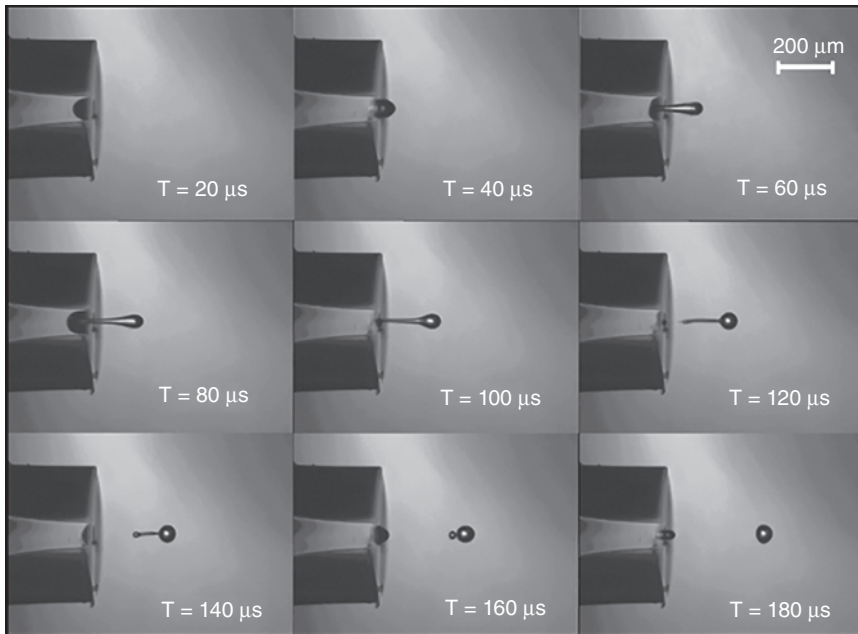
Figure 1.2 Jetting of a low viscosity ink (water) from a Microdrop Autopipette AK 510 with a nozzle of 70 \mu\text{m} . The print head is driven with a negative pulse. Initially the meniscus retracts and then the droplet is formed. The droplet speed is about 2 \text{ m s}^{-1} ; the droplet diameter is about equal to the nozzle diameter. Source: With permission from Microdrop GmbH Germany.
