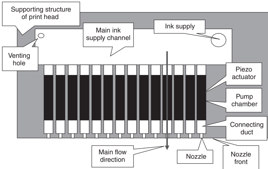
Figure 1.8 Basic layout of a closed end/open end multi-nozzle print head with pump chambers of which the length is large compared with the cross-sectional dimensions. The connecting duct towards the nozzle and the connection to the main ink supply channel may both have different cross-sectional dimensions compared with those of the pump section. The arrow symbolizes the main flow direction.
