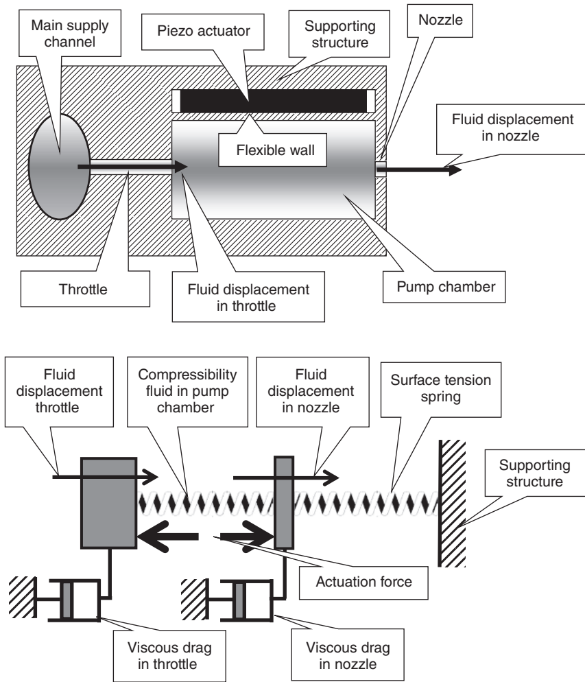
Figure 1.7 Schematic of single nozzle print head (or a specific pump out of a multi-nozzle print head) modelled as a two degrees of freedom oscillator. The oscillator has two masses, the mass of the fluid contained in the throttle and the mass of the fluid contained in the nozzle. The fluid in the nozzle is connected by a surface tension spring to the supporting structure and by another spring to the mass in the throttle by the compressibility of the fluid in the pump chamber. The fluid portions in the throttle and the nozzle undergo viscous drag upon motion. The actuator force works both on the mass in the throttle and the mass in the nozzle.
