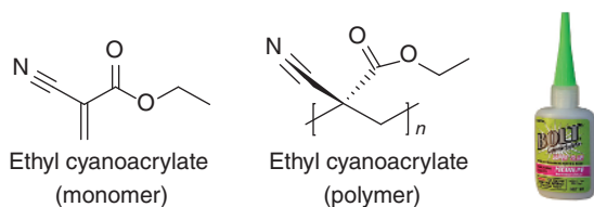
Figure 1.10 Chemical structures of the ethyl cyanoacrylate monomer and 'superglue' polymer. Source: BUPAK Ltd / Wikimedia Commons / public domain.
