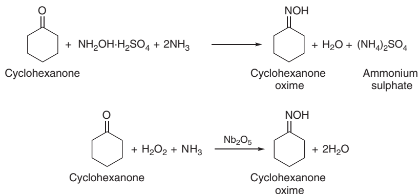
Figure 1.9 The classical ammximation route (top) and the new route improved by Shiju's catalyst, which avoids the ammonium sulphate by-product (bottom).
