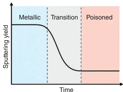
Figure 1.7 Time-resolved schematic of sputtering yield evolution in a Ti target under O_2 reactive sputtering, showing metallic, transition, and poisoned regimes.
