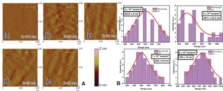
Figure 1.5 A: AFM images of pristine and 100 keV Ar + ion-irradiated Ge samples (a) pristine, (b) 3 \times 10^{17} , (c) 5 \times 10^{17} , (d) 7 \times 10^{17} , and (e) 9 \times 10^{17} ions/cm 2 irradiated samples (all images are in 5 μm × 5 μm scan size), B: shows the corresponding wavelength distribution. Source: [32] / Beilstein Journal of Nanotechnology / CC BY 4.0.
