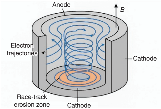
Figure 1.6 Illustration of electron trajectories in a magnetron showing confinement loops and race-track erosion zones.
