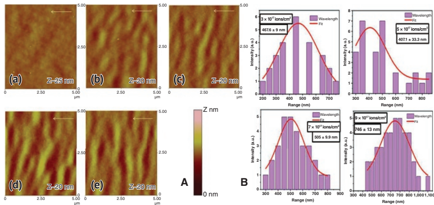
Figure 1.4 A: AFM images of pristine and 100 keV Ar + ion-irradiated Si samples (a) Pristine and irradiated samples with (b) 3 \times 10^{17} , (c) 5 \times 10^{17} , (d) 7 \times 10^{17} , and (e) 9 \times 10^{17} ions/cm 2 (all images are in 5 μm × 5 μm scan size) with corresponding wavelength distribution shown in B. Source: [32] / Beilstein Journal of Nanotechnology / CC BY 4.0.
