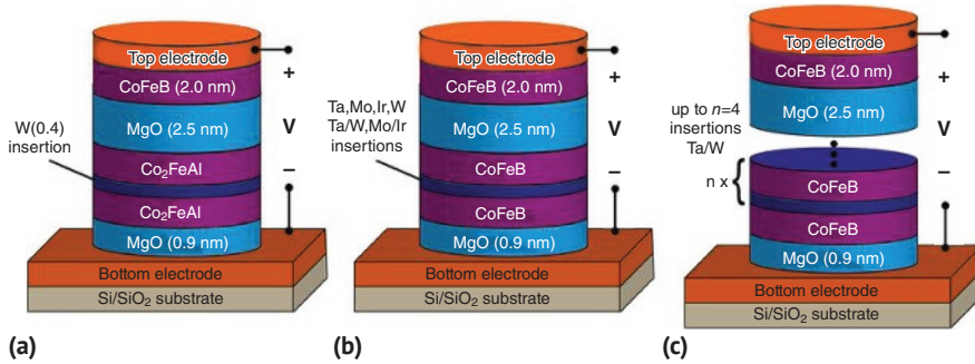
Figure 1.8 Schematic of the fabricated MTJs. (a)–(c) A SyF free layer is sandwiched by asymmetric double MgO barriers. The bottom electrode is Ta or W, and the top electrode is Ta/Pt. The Co 2 FeAl and CoFeB thicknesses in the SyF free layer varied from 0.5 to 1.5 nm for each stack by wedge across the wafer. Source: Reproduced from [56] / with permission of IOP Publishing.
