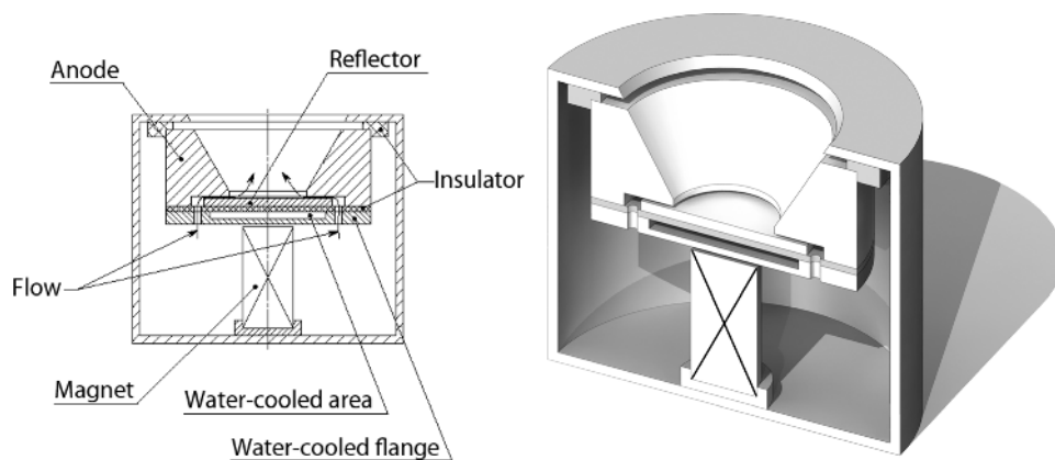
Figure 1.11 End-Hall with water-cooled anode through a dielectric plate; such design helps fast assembly [13].
