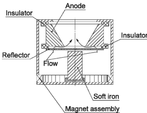
Figure 1.7 End-Hall with magnets at base; soft iron is used instead of magnet; design reduces temperature impact on magnets [9].
