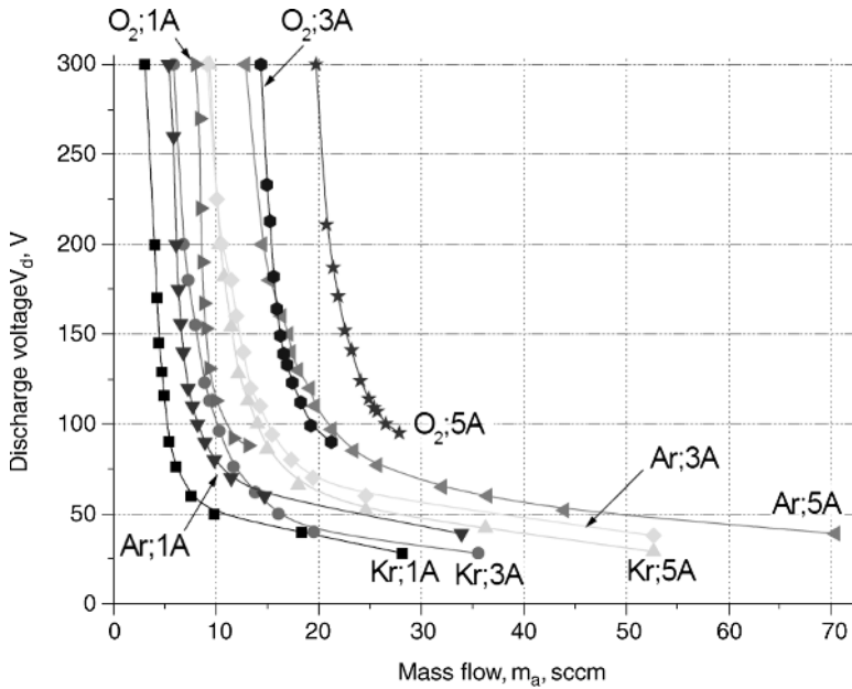
Figure 1.22 End-Hall ion source [21] discharge voltage as function of a working gas mass flow V_d = f(\dot{m}_a) at constant discharge currents I_d = 1, 3, 5 A for oxygen, argon and krypton.
