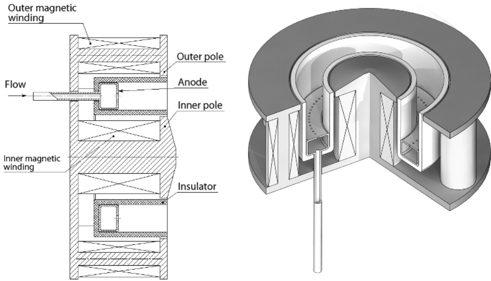
Figure 1.1 Magnetic layer closed drift ion source.
