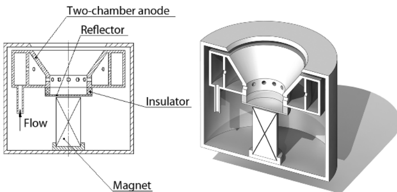
Figure 1.20 End-Hall with double-chamber anode and working gas through anode to improve ion beam energy distribution [21].
