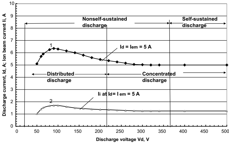
Figure 1.21 V–A characteristics, regimes, and modes for end-Hall ion source with discharge I_d and ion beam current I_i as functions of discharge voltage V_d for I_d = I_{em} = 5 A; working gas argon.
