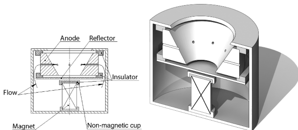
Figure 1.14 End-Hall with working gas through anode; protective cap over a magnet gives signal when ion beam goes through reflector [10].
