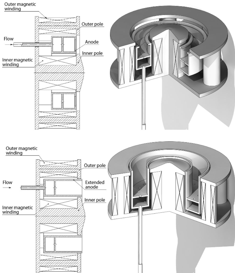
Figure 1.2 (a) Regular anode layer closed drift ion source. (b) Anode layer closed drift ion source with extended anode to reduce sputtering of magnetic poles.
