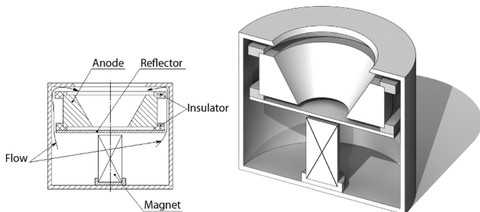
Figure 1.13 End-Hall with working gas applied from top, between anode and upper flange; low reflector's sputtering.
