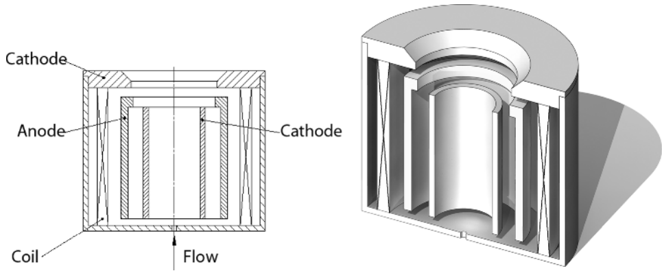
Figure 1.18 Hybrid end-Hall with anode layer ion source without external source of electrons [20].
