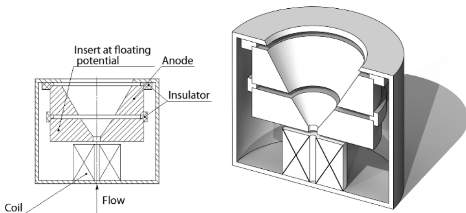
Figure 1.9 End-Hall with hollow insert under anode reduces insert's sputtering [11].
