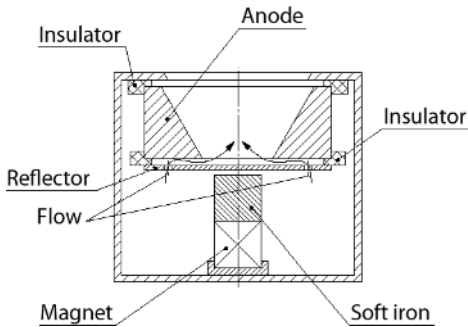
Figure 1.6 End-Hall with soft iron on top of permanent magnet to reduce temperature impact on magnet [8].
