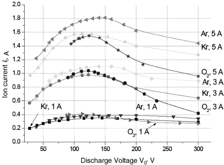
Figure 1.23 End-Hall ion source [21], ion beam current as function of discharge voltage I_i = f(V_d) at constant discharge currents I_d = 1, 3, 5 A for oxygen, argon and krypton.
