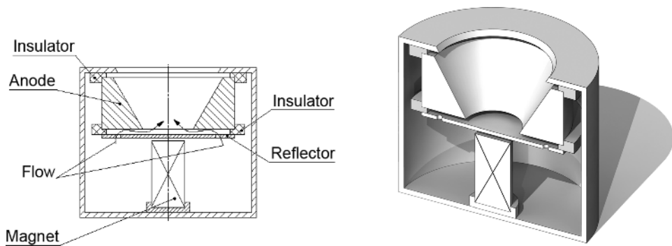
Figure 1.4 End-Hall ion source with permanent magnet on axis [7].
