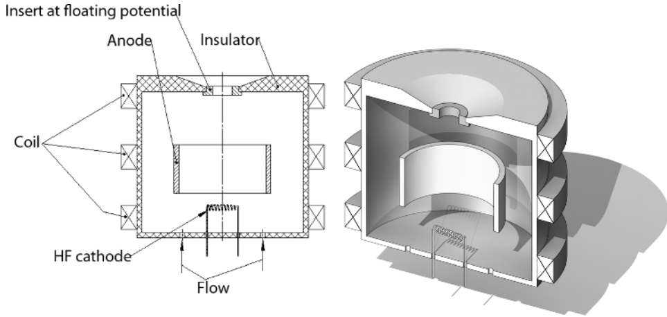
Figure 1.3 One of the first Hall-current low-energy ion sources [5]. HF cathode is in the discharge channel.
