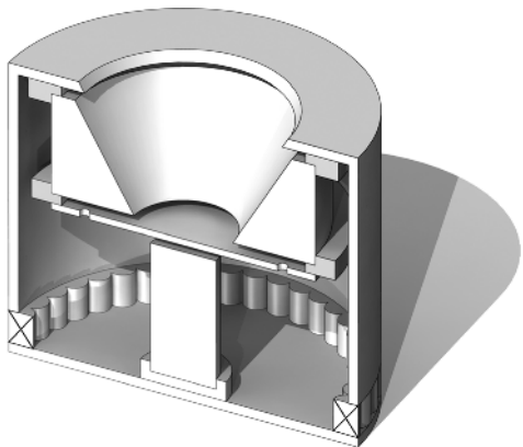
Figure 1.7 End-Hall with magnets at base; soft iron is used instead of magnet; design reduces temperature impact on magnets [9].
