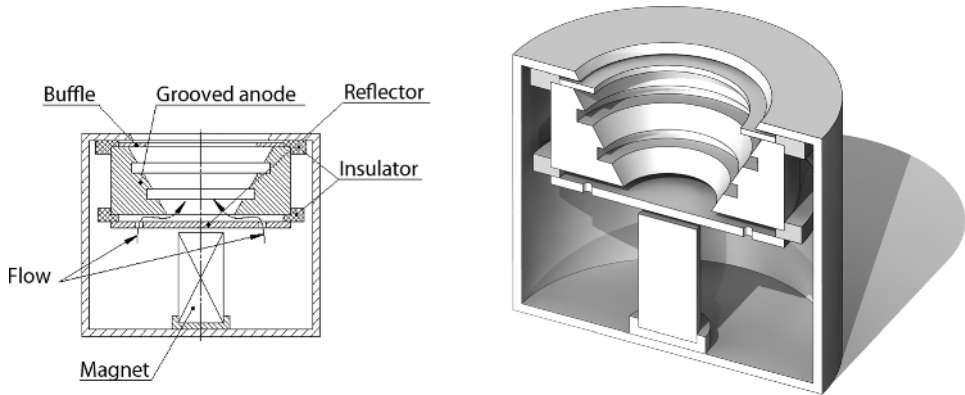
Figure 1.15 End-Hall with grooved anode and baffle to reduce anode “poisoning” [16].
