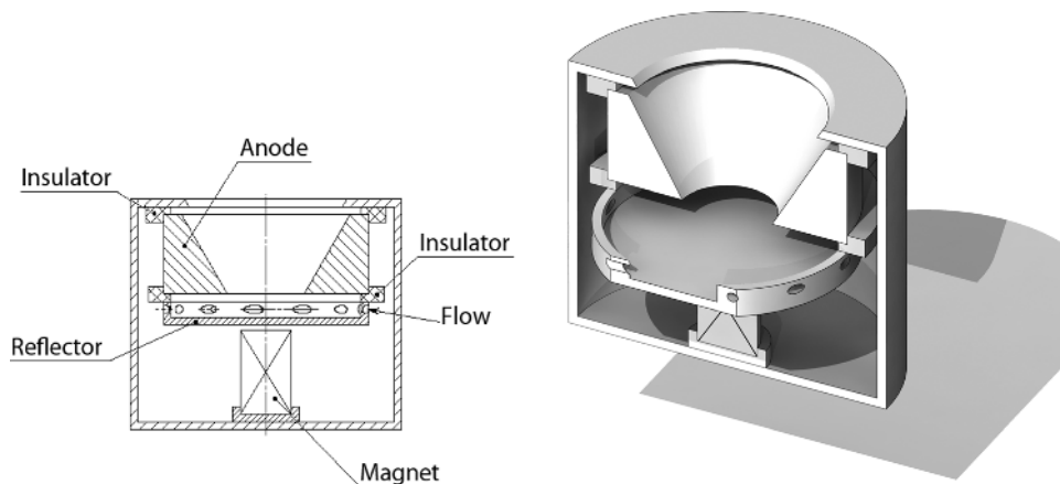
Figure 1.8 End-Hall with buffer area for improved gas distribution [10].
