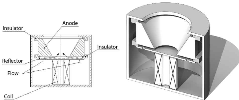
Figure 1.5 End-Hall ion source with magnetic coil on axis [7].
