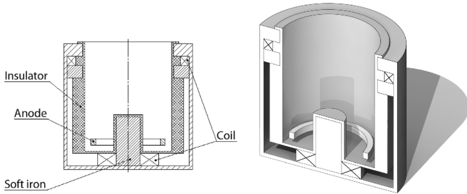
Figure 1.16 Hybrid end-Hall and closed drift ion source-thruster with electromagnets for magnetic field [18].
