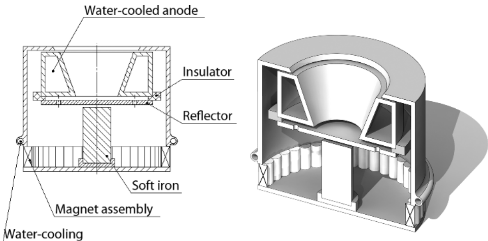
Figure 1.12 End-Hall with water-cooled anode and magnets helping stabilizing operating parameters [15].
