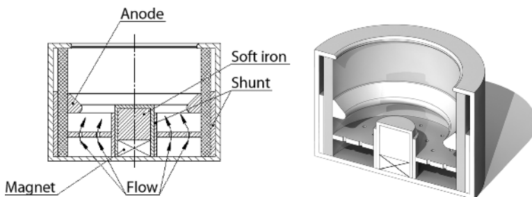
Figure 1.17 Hybrid end-Hall and Closed Drift ion source-thruster with permanent magnet soft iron and shunts for positive magnetic field gradient [19].
