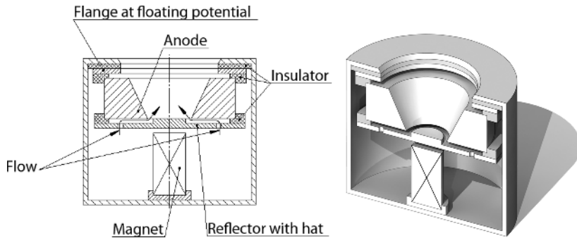
Figure 1.19 End-Hall with improved features: reflector with “hat”; floating potential flange to reduce ion beam spread.
