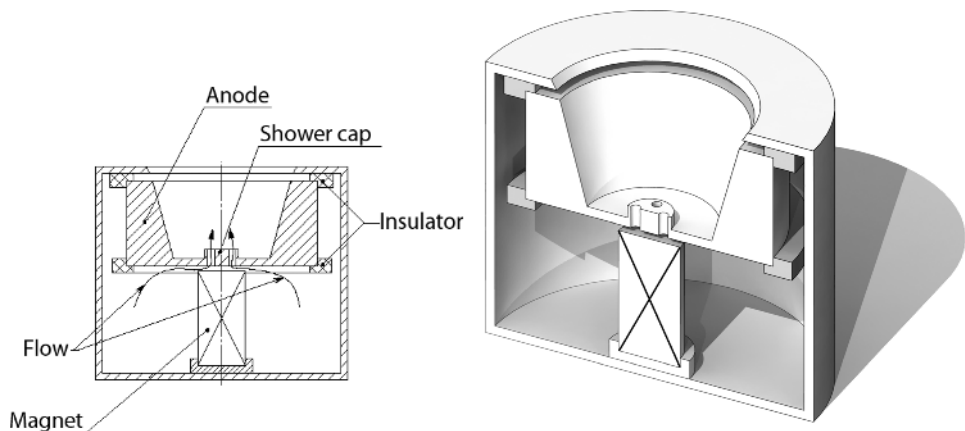
Figure 1.10 End-Hall with connected anode and reflector; working gas distributed through a “shower cap” [12].
