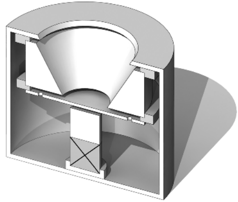
Figure 1.6 End-Hall with soft iron on top of permanent magnet to reduce temperature impact on magnet [8].
