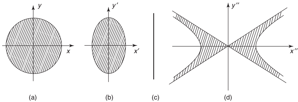
Figure 1.13 From non-restricted special relativity , also called “extended special relativity” [35, 103] one can recall the following. An intrinsically spherical (or point-like, at the limit) object appears in the vacuum as an ellipsoid contracted along the motion direction when endowed with a speed v < c . By contrast, if endowed with a speed V > c (even if the c -speed barrier cannot be crossed, neither from the left nor from the right), it would appear [35, 89, 103] no longer as a particle, but as occupying the region delimited by a double cone and a two-sheeted hyperboloid – or as a double cone, at the
