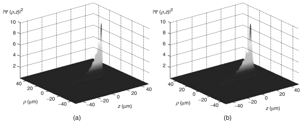
Figure 1.18 (a) A frozen wave with exponential growth, generated by the method in [87] through a superposition of Bessel beams, all with the same frequency
