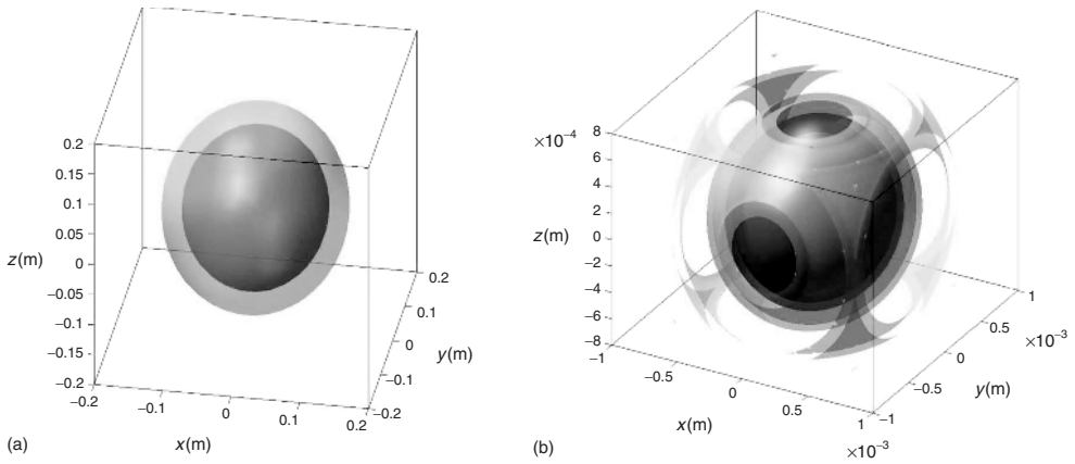
Figure 1.14 In Figure 1.13 we have seen how special relativity (SR), in its non-restricted version, predicted [89, 103] that, while the simplest subluminal object is obviously a sphere (or, in the limit, a space point), the simplest superluminal object is, on the contrary, an X-shaped pulse (or, in the limit, a double cone). The circumstance that the localized solutions to the wave equations do follow the same pattern is rather interesting, and is expected to be useful – in the case, for example, of elementary particles and quantum physics –
