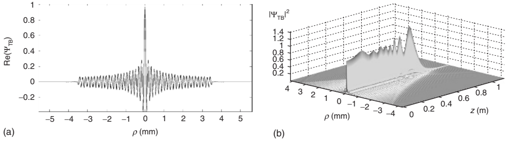
Figure 1.8 (a) Field given by Equation 1.47, Equation 1.51, with q = 0 , L = 3R^2 , q_R = 6/L , and N = 23 . (b) Intensity of a Bessel beam truncated by a finite aperture, as given by solution (1.43).
