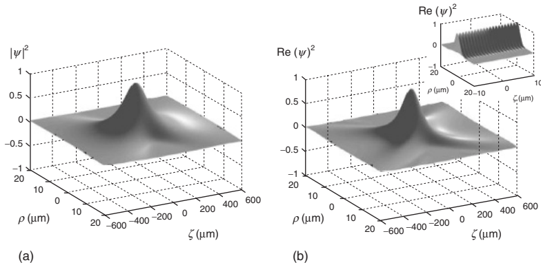
Figure 1.4 The intensity of the (a) complex and (b) real part of a quasi-monochromatic, totally “forward,” superluminal optical focus wave mode pulse, with V = 1.5c , \alpha_0 = 1.256 \times 10^7 \text{ m}^{-1} and s = 1.194 \times 10^{-4} \text{ m} , which correspond to \omega_{\min} = 3.77 \times 10^{15} \text{ Hz} , and \Delta\omega = 3.77 \times 10^{12} \text{ Hz} , that is to a picosecond pulse with \lambda_0 = 0.5 \text{ }\mu\text{m} .
