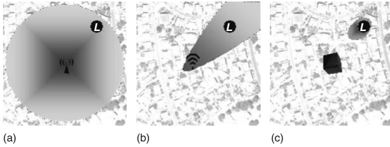
Figure 1.11 Areas covered by the electromagnetic (or acoustic) signals in the case, once more, of (a) omnidirectional transmission, (b) standard directional transmission, and (c) spot-to-spot signal transmission permitted by our frozen wave techniques. (Courtesy of Andrei Utkin.)
