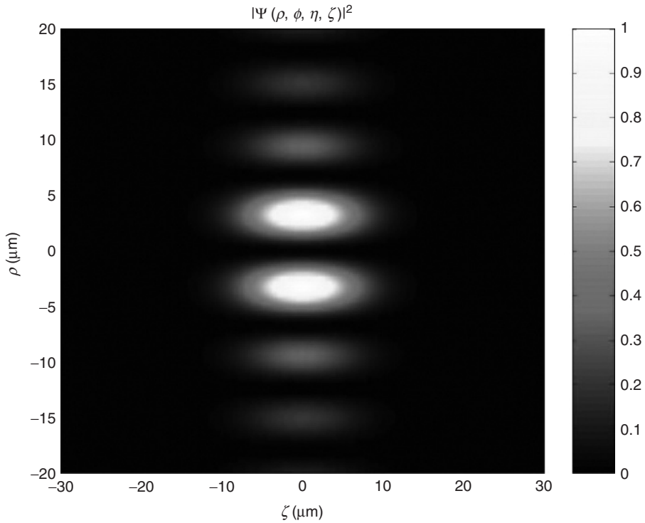
Figure 1.15 Orthogonal projection of the field intensity corresponding to the higher order subluminal pulse represented by the exact solution Equation 1.93, quantity \Psi being given by Equation 1.69 with the Gaussian spectrum (1.70). This time, the pulse intensity happens to have a “donut”-like shape.
