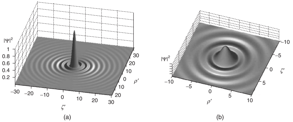
Figure 1.21 Here, and in Figure 1.22, we depict the square magnitude of elementary solutions of the type (1.119), corresponding to the real spectrum S(u) = s_0 \exp [(E - E_+)a] , as a function of \rho' \equiv \rho\sqrt{P}/\hbar and of \zeta' \equiv \zeta\sqrt{P}/\hbar . Quantity a is a positive number (when a = 0 one ends up with a solutions similar to Mackinnon's [31]), while b for simplicity has been chosen equal to zero. (a) Corresponds to a = E_+/5 . For (b), normalized
