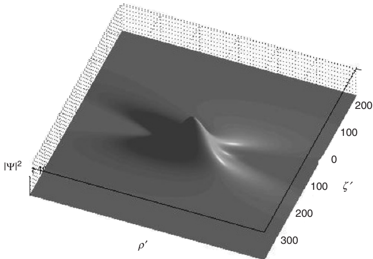
Figure 1.22 The solution, under all the previous conditions, with an increased value of \bar{A} , namely with \bar{A} = 20 . An X-shaped structure more evidently appears, contributing in a more clear way to the general form of the solution (see the text).
