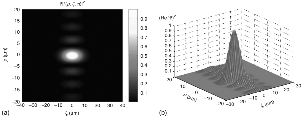
Figure 1.9 (a) The intensity orthogonal projection for a pulse corresponding to Equations 1.70 and 1.71 in the case of an optical frequency, namely for a subluminal pulse with velocity v = 0.99 c , carrier angular frequency \omega_0 = 2.4 \times 10^{15} Hz (i.e., \lambda_0 = 0.785 \mu\text{m} ) and FWHM bandwidth (that is, full width at half maximum) \Delta\omega = \omega_0/20 = 1.2 \times 10^{14} Hz, which results in an optical pulse of 24 fs. One has also
