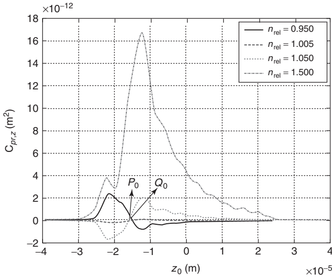
Figure 1.19 Radiation pressure cross-section exerted on a spherical dielectric particle of radius a = 3.75 \mu\text{m} as a function of its relative refractive index and of the distance z_0 from z = 0 . The external medium is assumed to be water. Points of longitudinal stable equilibrium are denoted by P_0 and Q_0 .
