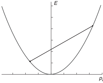
Figure 1.20 The allowed region is the one internal to the parabola, since (to avoid divergencies) it must be E \geq p_z^2/(2m) . In this case, the parabola and the chosen straight-line have equations E = p_z^2/(2m) and
