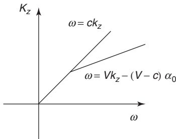
Figure 1.3 The Dirac delta function in Equation 1.32 confines the spectral parameters \omega, k_z of the Bessel beams to the straight line \omega = V k_z - (V - c)\alpha_0 , with \alpha_0 > 0 .
