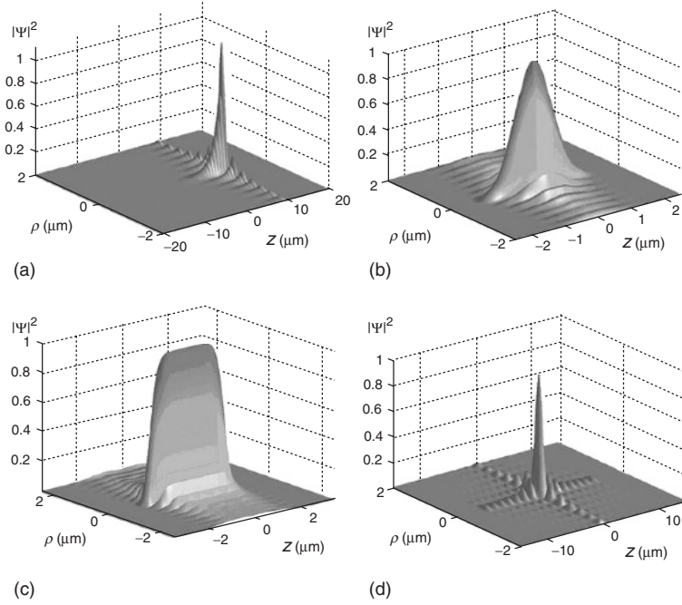
Figure 1.12 Frozen waves with the on-axis longitudinal field pattern chosen as (a) exponential, (b) Gaussian, (c) super-Gaussian, and (d) zero-order Bessel function.
