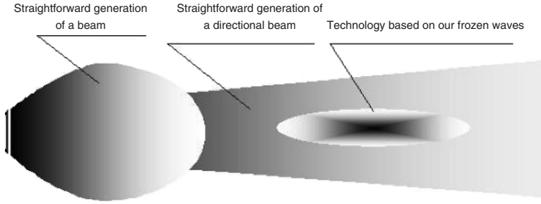
Figure 1.10 See the explications contained in the figures themselves, which apparently refer to ordinary (electromagnetic or acoustical) transmission, to standard directional transmission, and to well-localized transmission allowed by our frozen wave techniques. (Courtesy of Andrei Utkin.)
