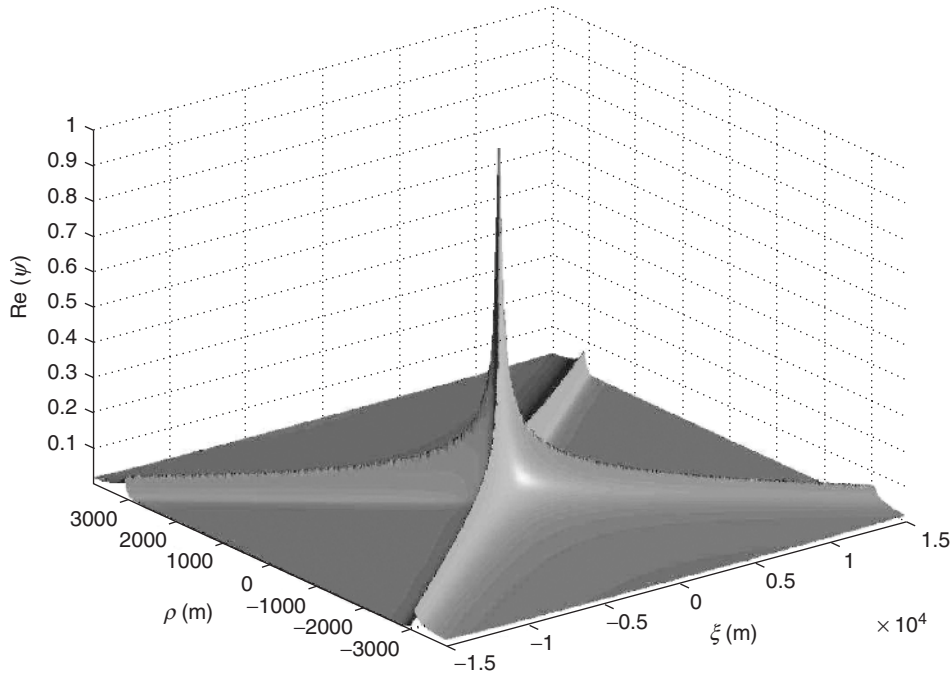
Figure 1.1 Plot of the real part of the ordinary X-wave, evaluated for V = 1.1c with a = 3 m.
