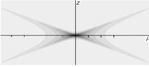
Figure 1.2 All the X-waves (truncated or not) must have a leading cone in addition to the rear cone, such a leading cone having a role even for the peak stability [9]. Long ago, this was also predicted, in a sense, by (non-restricted [1, 13, 14]) special relativity: one should not forget, in fact, that all wave equations, and not only Maxwell's, have an intrinsic relativistic structure. By contrast, the fact that X-waves have a conical shape induced some authors to look for (untenable) links – let us now confine ourselves to
