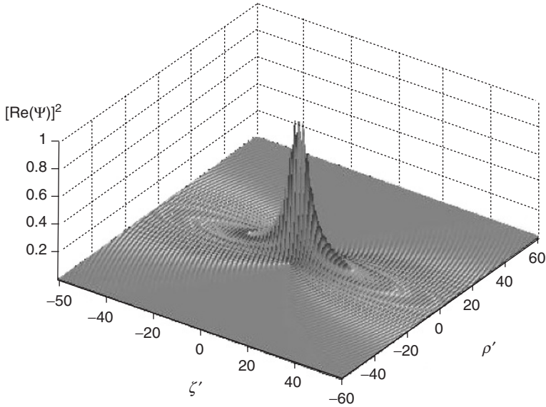
Figure 1.23 The (square of the) real part of \Psi shows, in three-dimension, also some “internal oscillations”. This Figure corresponds, for example, to the value \bar{A} = 5 .
