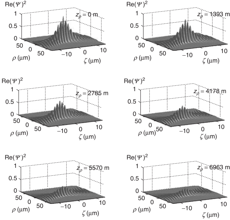
Figure 1.6 The space–time evolution, from the pulse’s peak at z_p = 0 to z_p = Z , of a totally “forward,” finite-energy, superluminal non-diffracting wave optical pulse represented by Equation 1.37, with the following parameter values: a = 20 m, s = 3.99 \times 10^{-6} m (note that a \gg s ), V = 1.005c and \alpha_0 = 1.26 \times 10^7 m ^{-1} .
