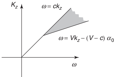
Figure 1.5 The spectrum (1.35), when written in terms of the spectral parameters \omega and k_z , has its domain indicated by the shaded region.
