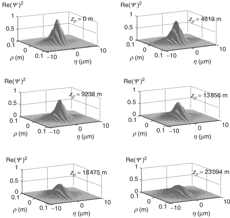
Figure 1.7 The space–time evolution, from the pulse’s peak at z_p = 0 to z_p = Z , of a totally “forward,” finite-energy, luminal non-diffracting wave optical pulse represented by Equation 1.37, with a = 1.59 \times 10^{-6} m, s = 1 \times 10^4 m (note that s \gg a ), V = 1.5c , \alpha_0 = 1.26 \times 10^7 m ^{-1} .
