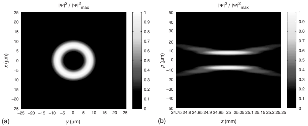
Figure 1.16 (a) Transverse section at z = L/2 of the considered higher-order FW. (b) Orthogonal projection of the three-dimensional intensity pattern of the same
