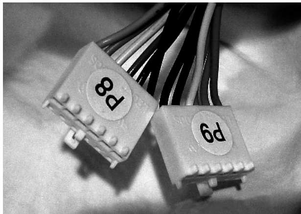
FIGURE 1.39 AT power supply system board connectors
