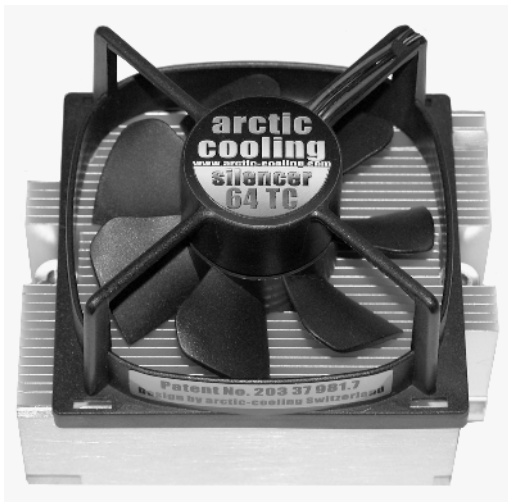
FIGURE 1.73 An active hard disk cooler
