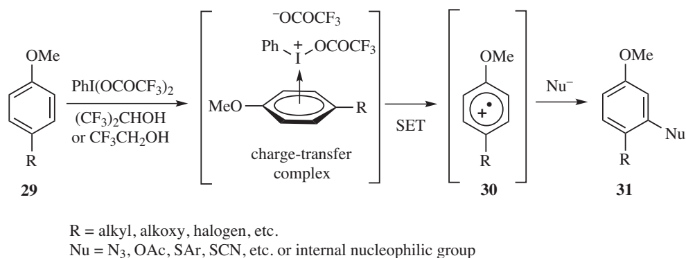
Scheme 1.5 Simplified single-electron transfer (SET) mechanism for the reaction of p -substituted phenol ethers with [bis(trifluoroacetoxy)iodo]benzene.
