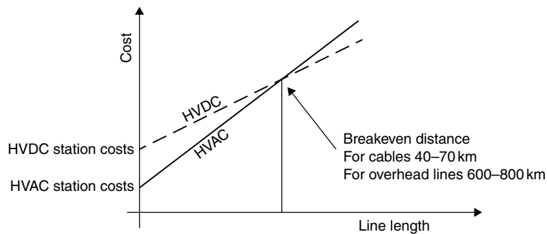
Figure 1.1 HVDC and HVAC transmission cost comparison.
