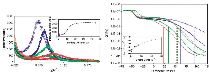
Figure 1.13 Influence of the binding constant of telechelic supramolecular polymers on phase separation as observed with SAXS and corresponding rheological analysis. Reprinted with permission from the American Chemical Society [50].
