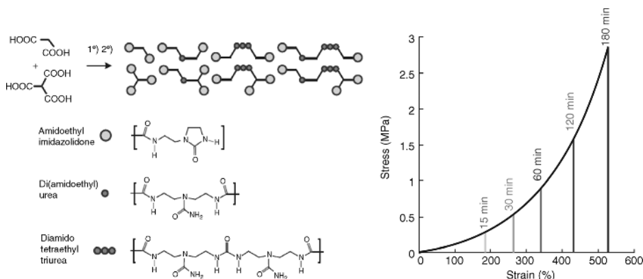
Figure 1.12 A supramolecular rubber based on hydrogen bonding generates a self-healing material at room temperature. The mechanical properties recover in time as the hydrogen-bonding network is restored. Reprinted with permission from Nature Publishing Group [45a].
