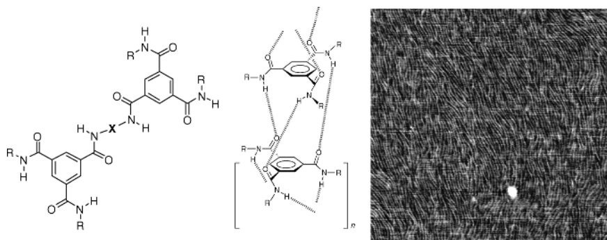
Figure 1.20 Supramolecular polymers based on the benzene-1,3,5-tricarboxamide motif (left) and the nano-fibers as observed with AFM (phase image, 450 \times 450 nm, right). Reprinted with permission from the American Chemical Society [59].
