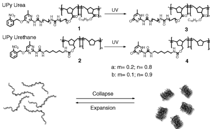
Figure 1.21 The creation of supramolecular nano-particles based on intramolecular cross-linking via hydrogen bonding. Reprinted with permission from the American Chemical Society [61a].
