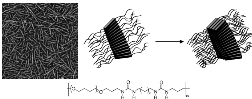
Figure 1.11 Atomic force microscopy phase image ( 500 \times 500 nm) of nano-fibers as observed in thermoplastic elastomers based on the bis-urea motif (left) and the schematic
