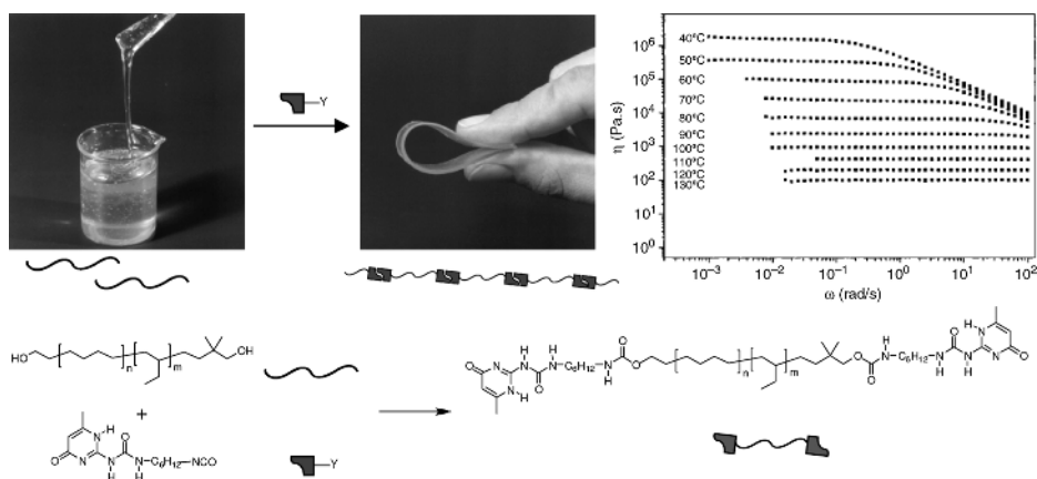
Figure 1.15 A supramolecular thermoplastic elastomer obtained by functionalization of a short telechelic poly(ethylene-butylene) oligomer with an ureido-pyrimidinone
