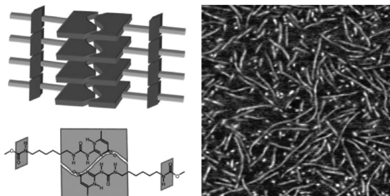
Figure 1.16 Schematic representation of the lateral interactions creating supramolecular crosslinks (left) and the nanofibers as visualized with AFM ( 500 \times 500 nm phase image). Reprinted with permission from Wiley-VCH [54b].
