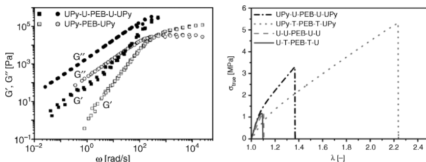
Figure 1.17 Rheological master curves (left) and tensile testing (right) of various telechelic supramolecular poly(ethylene-butylene) polymers. Reprinted with permission from the American Chemical Society [53].
