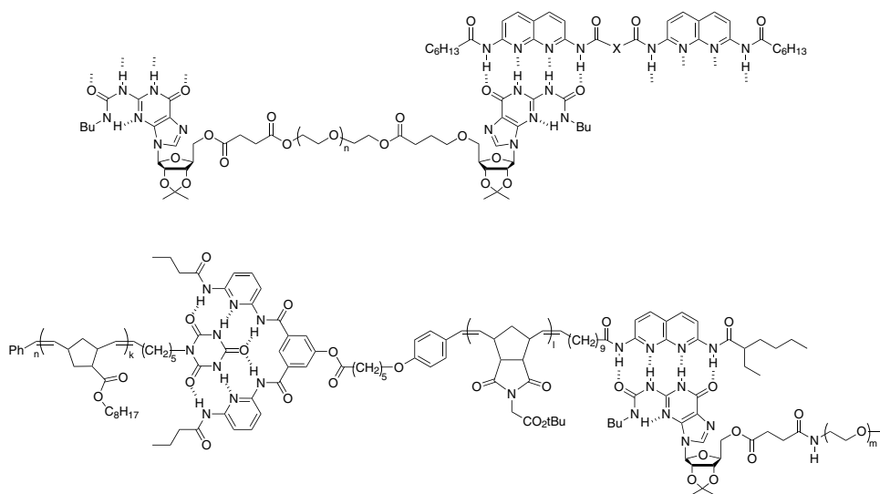
Figure 1.8 Alternating (top) and triblock (bottom) supramolecular copolymers created in solution by using the directionality of complementary hydrogen-bonding motifs [28b,29].
