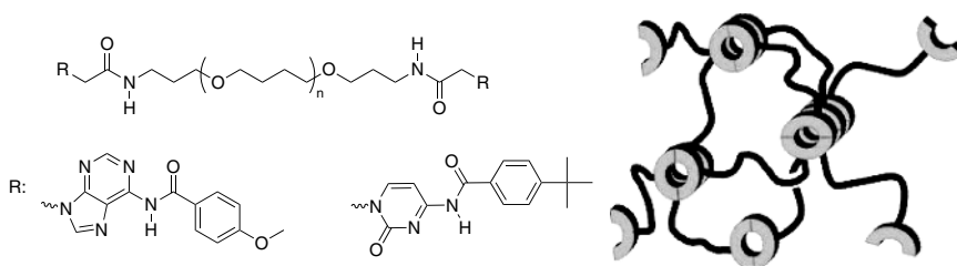
Figure 1.14 Nucleobase hydrogen-bonded supramolecular polymers and their schematic aggregation into phase-separated hard segments. Reprinted with permission from the American Chemical Society [51b].
