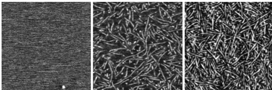
Figure 1.18 AFM phase images ( 500 \times 500 nm) of UPy-PEB-UPy, UPy-T-PEB-T-UPy and UPy-U-PEB-U-UPy respectively.
