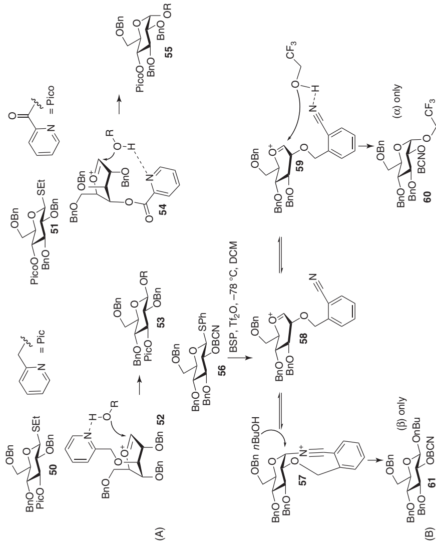
Scheme 1.10 (A) Hydrogen-bonding acceptor delivery by picolinyl and picolinyl ether; (B) hydrogen-bonding acceptor delivery by cyanobenzyl ethers.
