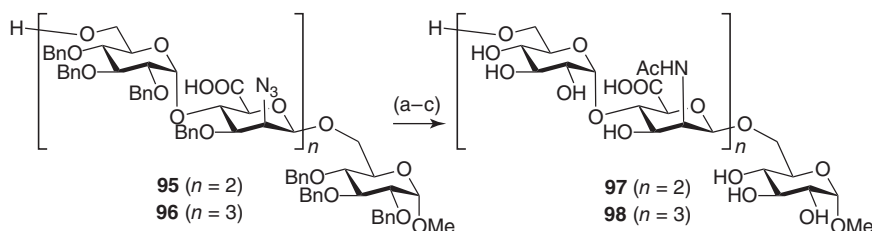
Scheme 1.15 Birch reduction of teichuronic acid oligosaccharides in which cleavage of the mannosaminuronic acid linkages was encountered; (a) Na (s), liquid \text{NH}_3 , and THF, -60^\circ\text{C} ; (b) HPLC purification; (c) \text{Ac}_2\text{O} , \text{NaHCO}_3 , and THF/ \text{H}_2\text{O} ( 97 : 35% over 2 steps; 98 : 14% over 2 steps).
