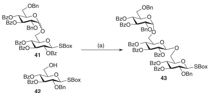
Scheme 1.8 Neighboring group participation-assisted selective activation: (a) \text{Cu}(\text{OTf})_2 , \text{TfOH} , and \text{DCM} (70%).
