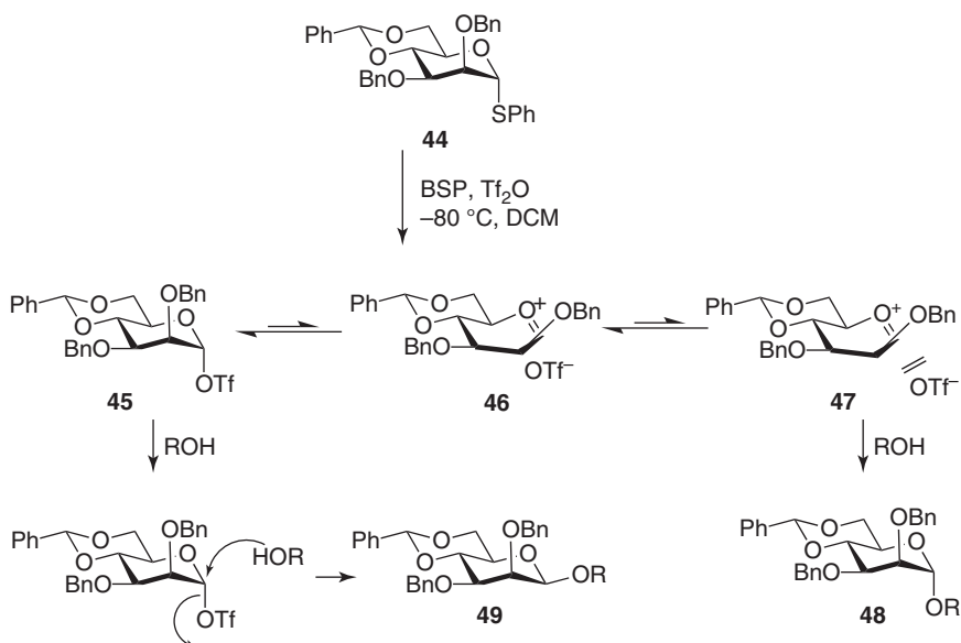
Scheme 1.9 Reaction mechanism manifold to account for the stereoselectivity in glycosylation reactions of benzylidene mannoside donors.
