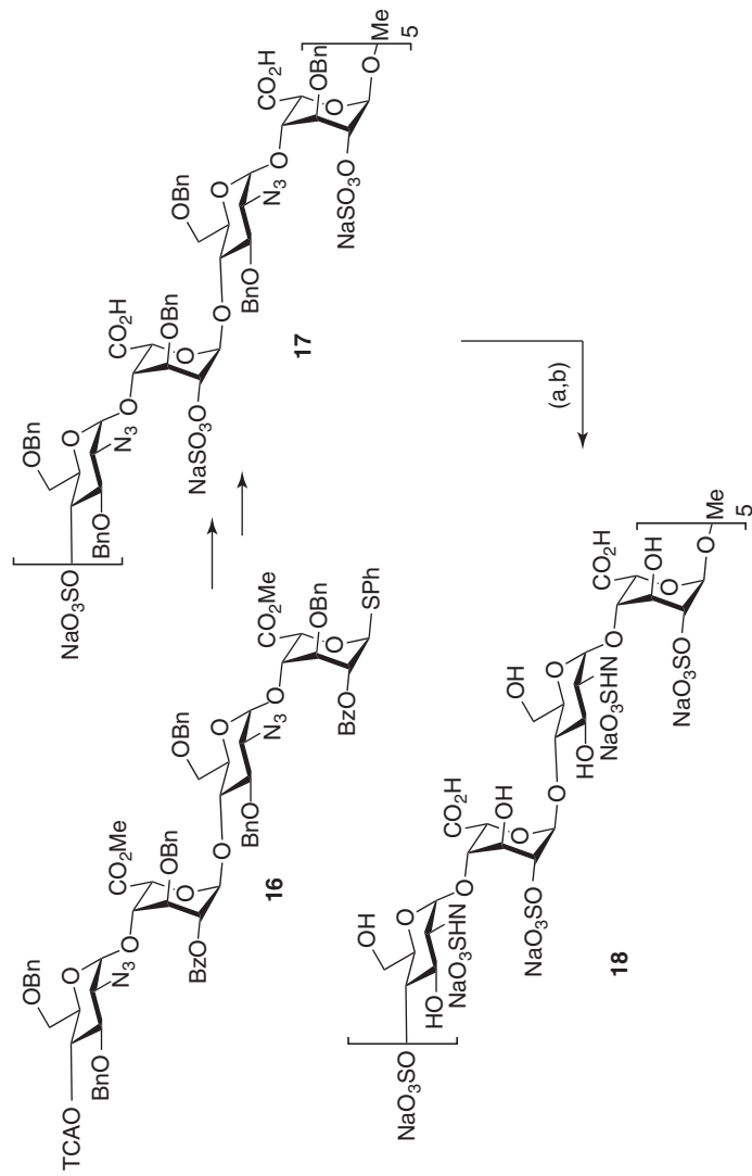
Scheme 1.4 Block coupling to heparin-like 20-mers. (a) \text{Pd}(\text{OH})_2/\text{C} and \text{EtOH}/\text{H}_2\text{O} (89%); (b) \text{SO}_3 -Pyridine and \text{H}_2\text{O} .
